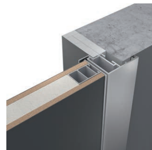
U-SYSTEM frame without adjustment panel
