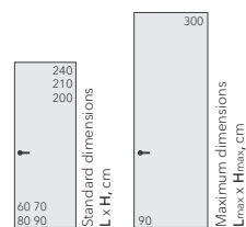
U-SYSTEM frame Installation in an finished opening
