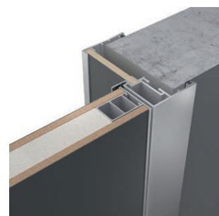
U-SYSTEM frame with adjustment panel
