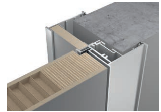
PLANAR frame
